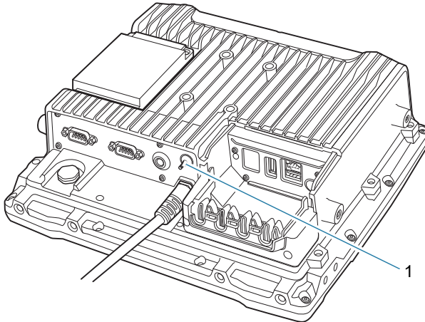
Figure 7 Ground Lug
