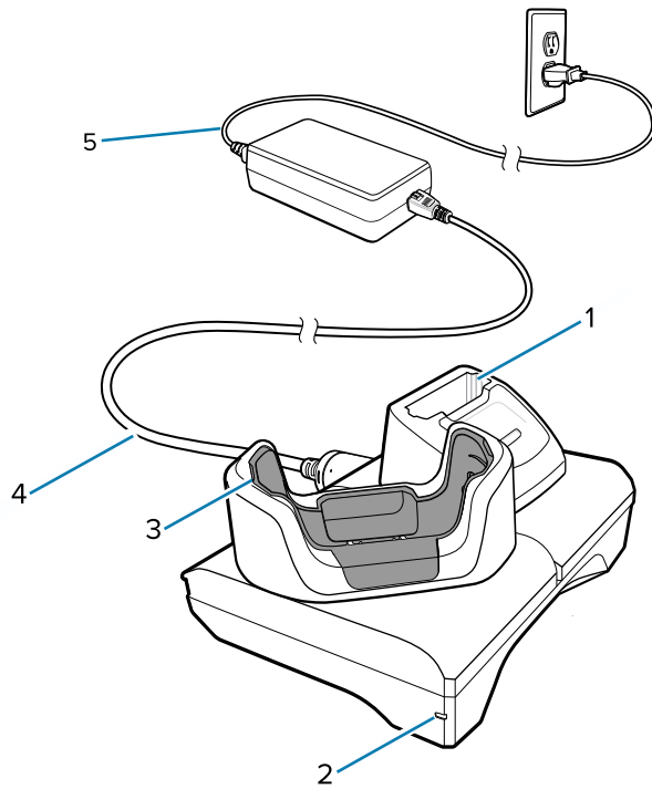
Figure 32 2-Slot USB Charge Cradle
