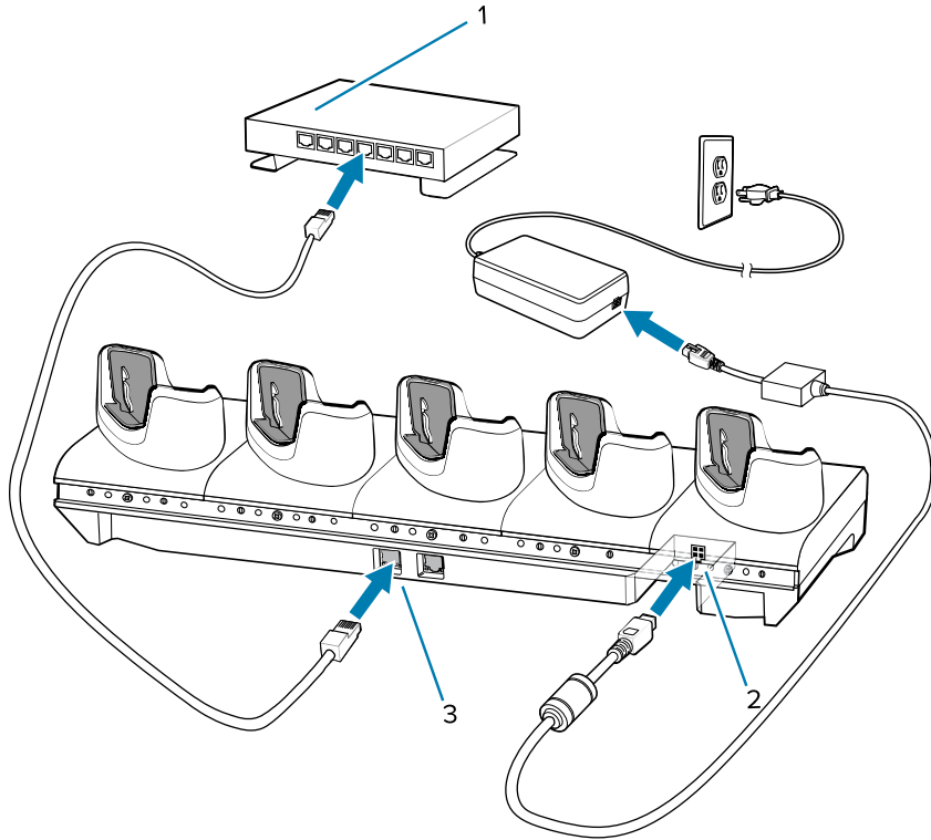
Figure 34 5-Slot Ethernet Cradle
