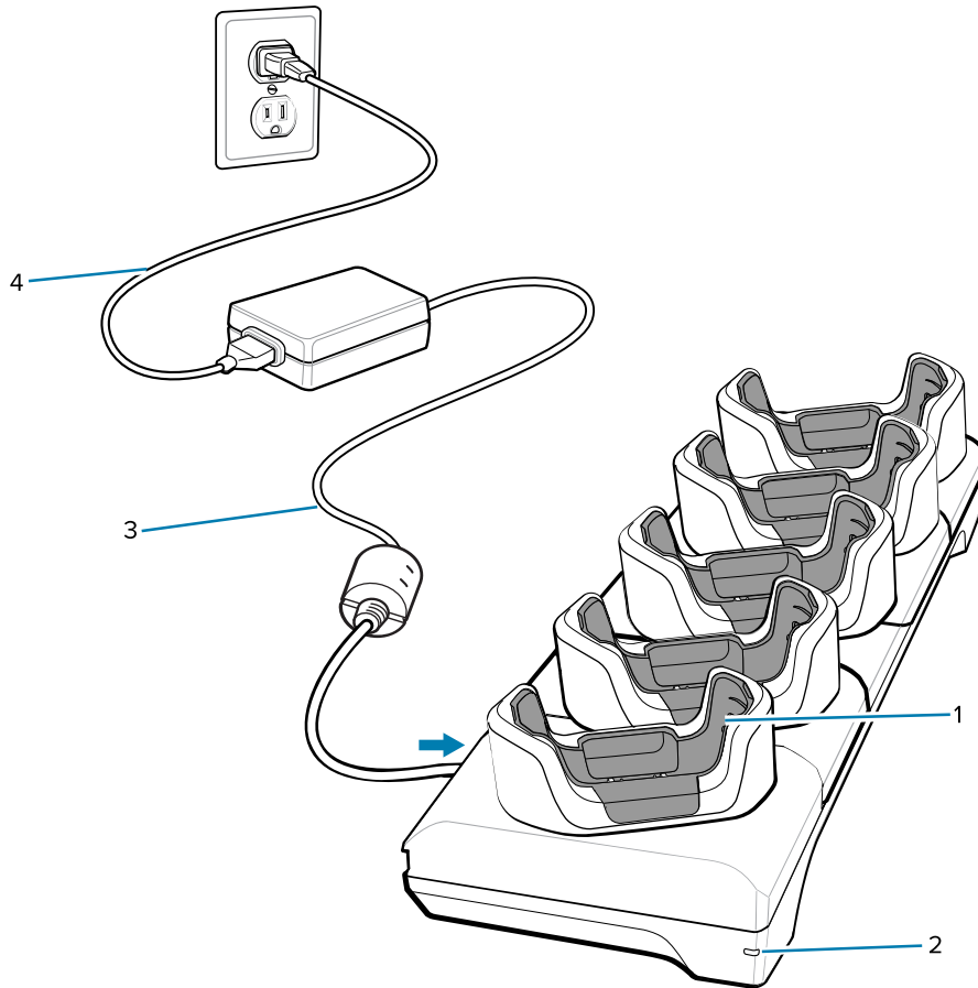
Figure 33 5-Slot Charge Only Cradle
